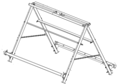
Support for 10 cylinders
